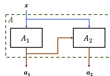
Figure 1: The composition of two algorithms (solid boxes), viewed as a single larger algorithm A (dashed box).
